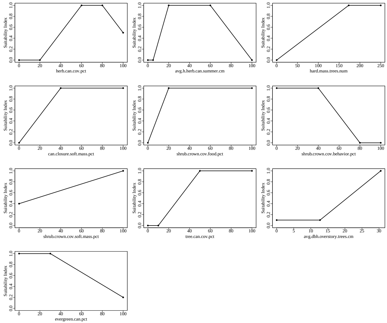
Figure 1. Suitability index graphs for variables included in the easternwildturkeyForestHardDBH30.5cm model in ecores.
